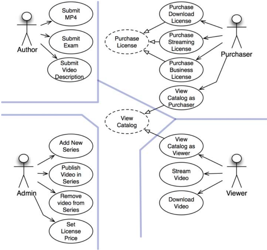
Figure 33.1 A typical use-case analysis
