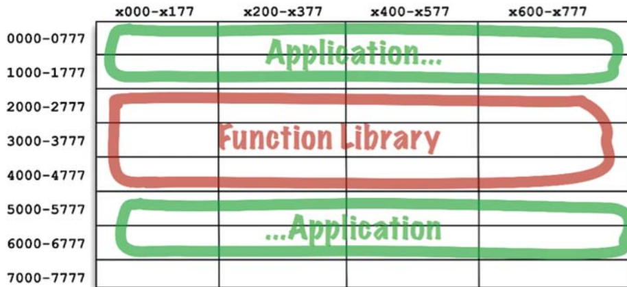
Figure 12.2 Splitting the application into two address segments
