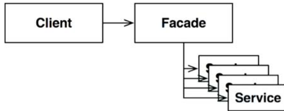
Figure 24.2 The Facade pattern
